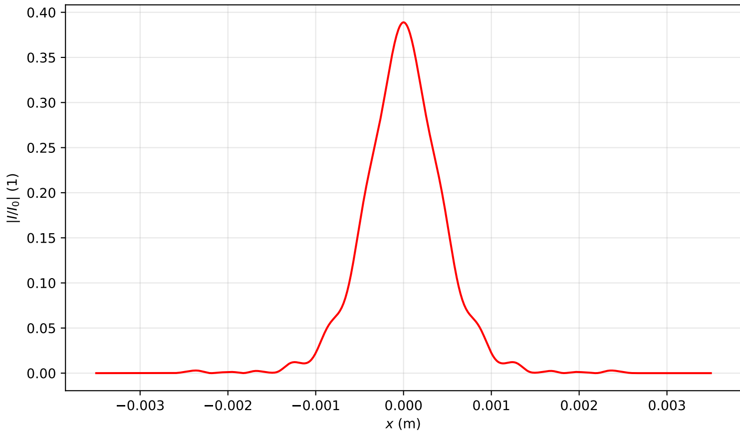
Intensity profile I(x, y = 0, z = 2.707)/I_0 , P_{in}=1.0P_{cr} , artificial time
